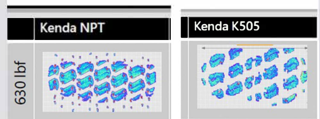
Footprint study of Kenda 24" NPT vs benchmark K505 and competitors
